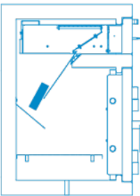
Deposit falls securely into the vault
