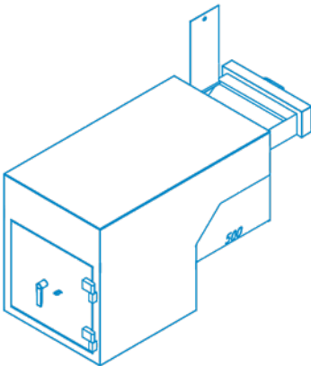
Customised drawer at the back (with up to 500 mm overhang possible)
